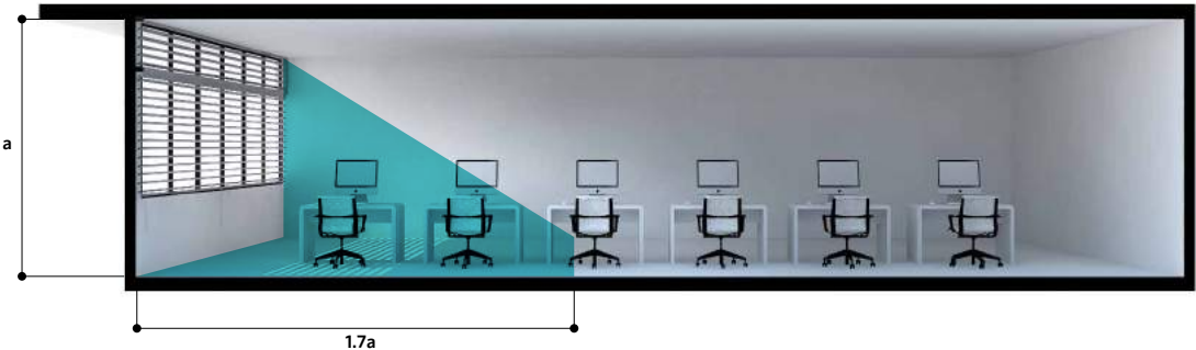
FIGURE 4.5.4 | DAYLIGHT FACTOR OF 1% IS FOUND AT A DISTANCE OF APPROXIMATELY 1.7a WHEN HORIZONTAL BLINDS ARE USED TO PROVIDE GLARE PROTECTION
