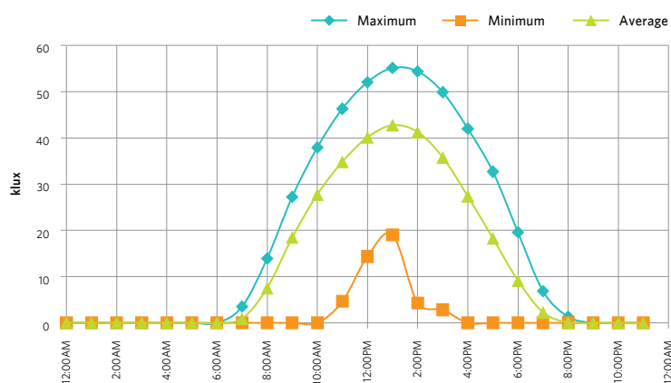
CHART 4.1 | DIFFUSE DAYLIGHT AVAILABILITY FROM THE TEST REFERENCE YEAR (TRY) WEATHER DATA
