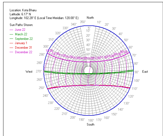
CHART 2.1.5 | SUN-PATH OF KOTA BHARU
